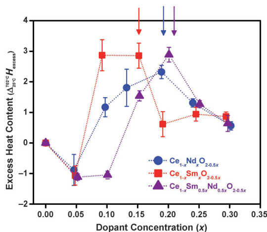
Figure 4. Excess heat contents of NDC, SDC, and SNDC ( 0.05 \leq x \leq 0.30 ) from room temperature to 702 °C. \Delta_{25^\circ\text{C}}^{702^\circ\text{C}}H_{xs} with respect to dopant concentration. The arrows mark the critical dopant concentrations that yield the maximum defect disordering near 700 °C for a given solid solution.
